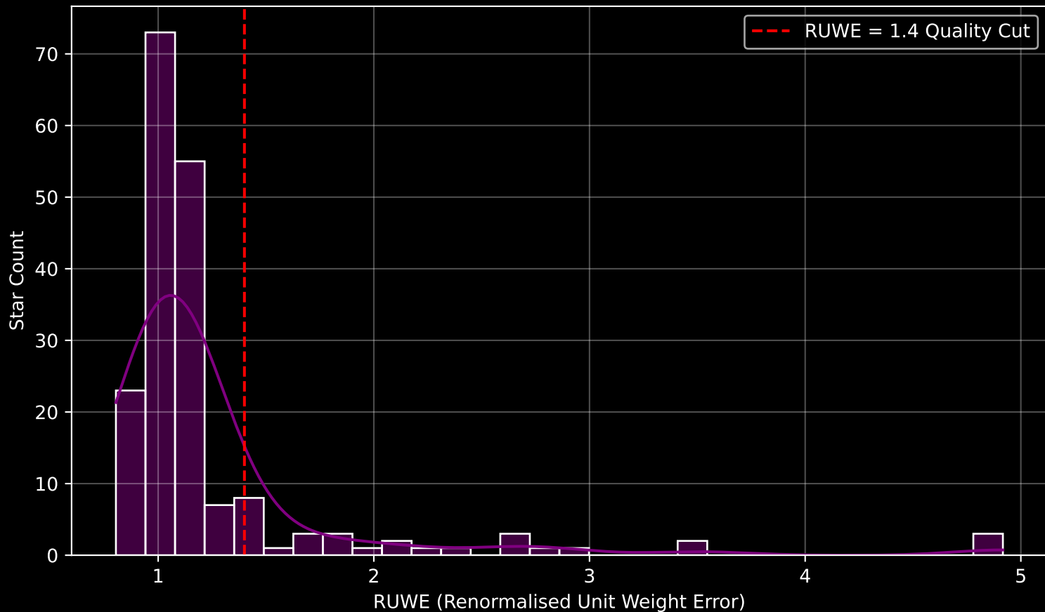
GAPOGEE DR17 Field [177+32] RUWE Distribution (n= 188)
