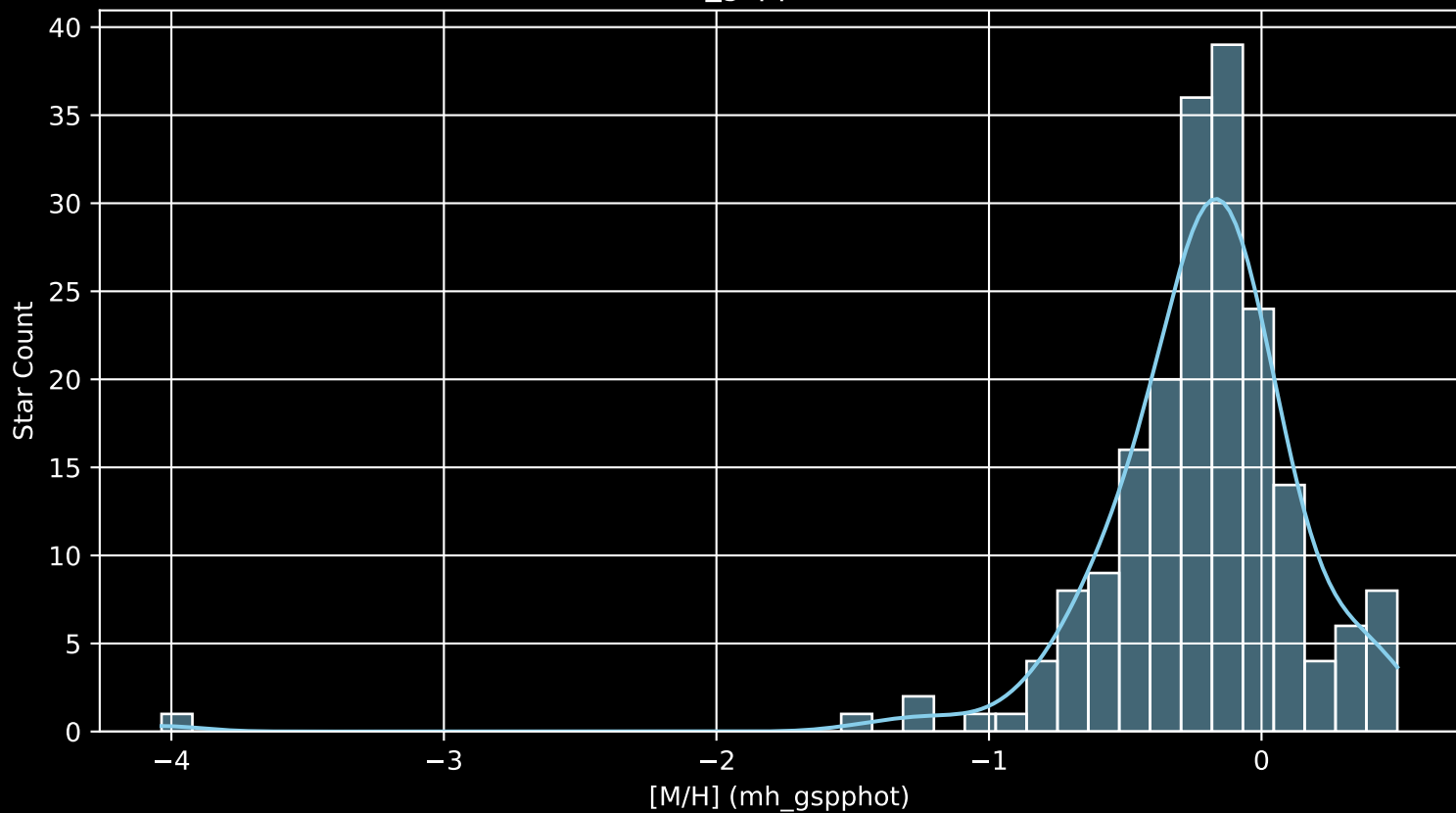
APOGEE DR17 Field: [177+32 [M/H] (mh_gspphot) (n= 194)
