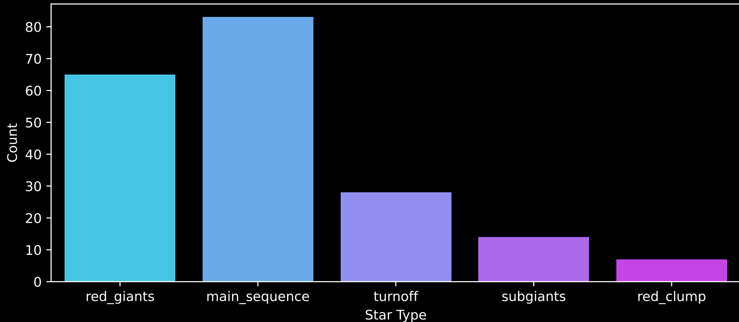
APOGEE DR17 Field: [177+32] Count plot of Star Type
