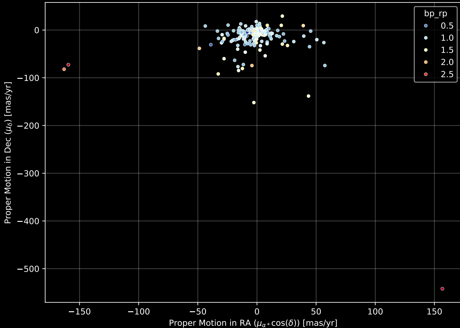
APOGEE DR17 Field: [177+32] Proper Motion Diagram (n= 197)
