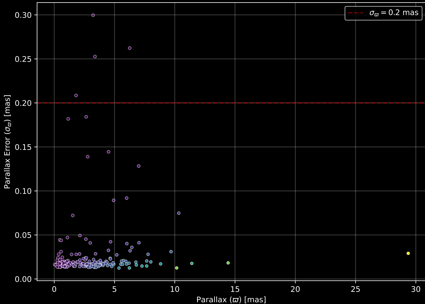
APOGEE DR17 Field: [177+32] Parallax Quality (n= 197)
