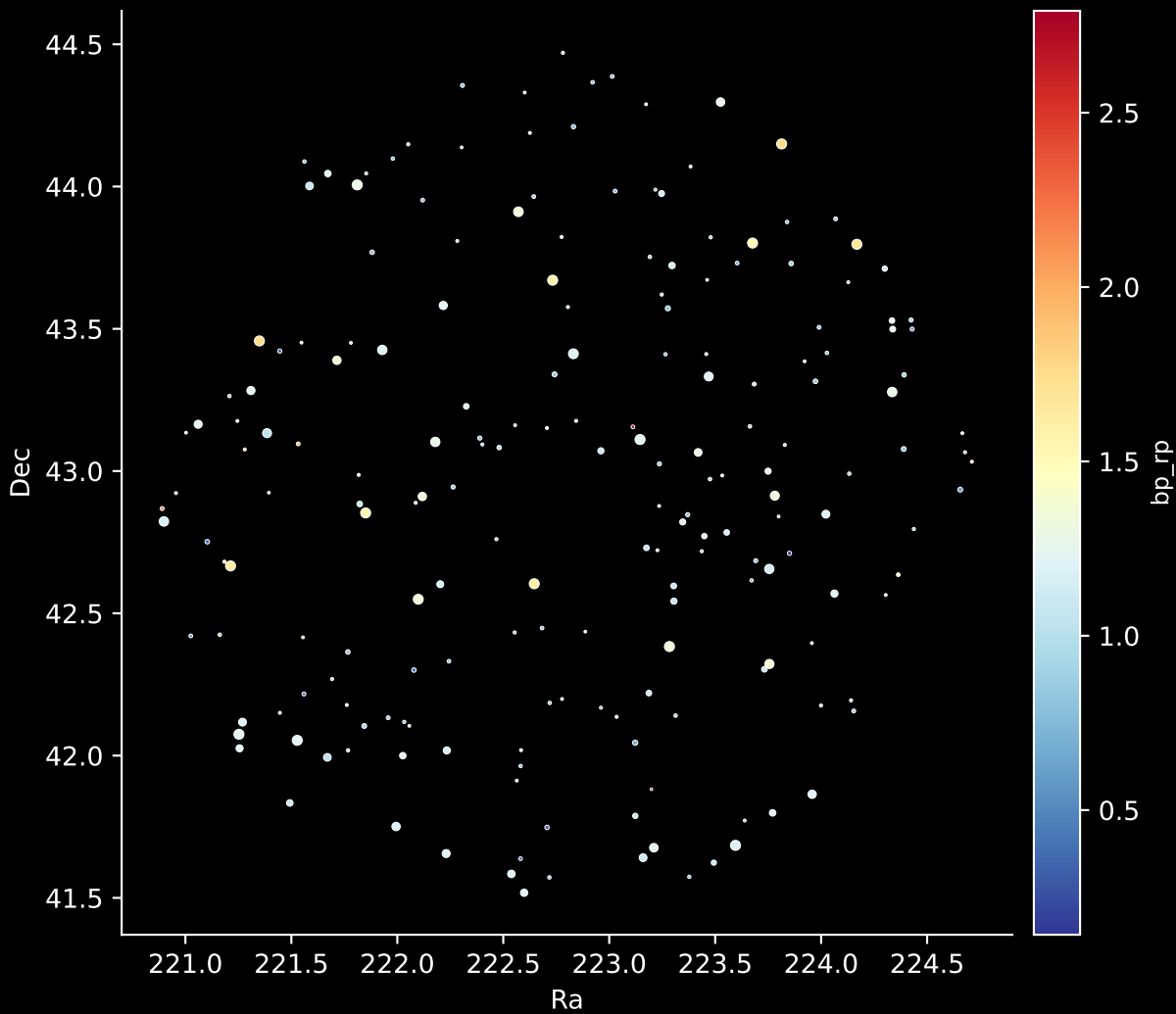
APOGEE DR17 Field: [177+32] Stars: 197
